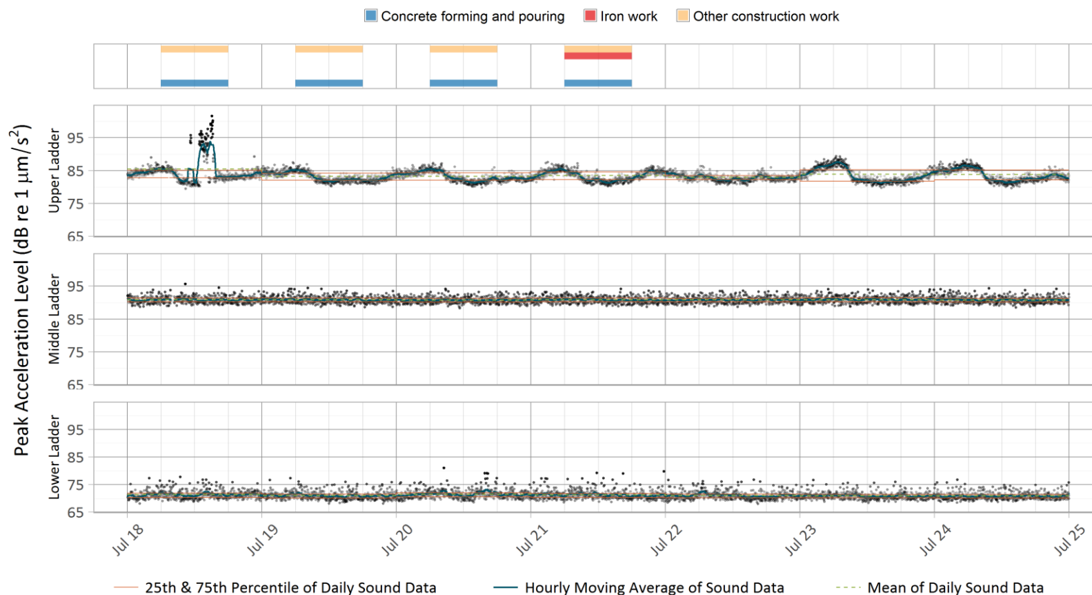
Figure 9 Peak Acceleration Levels Measured by Triaxial Accelerometers with Construction Information for Week 29
