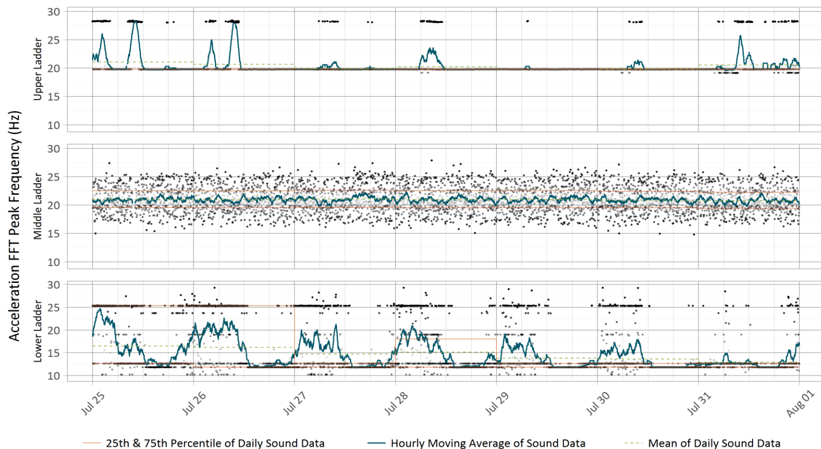
Figure 2 Acceleration Peak Frequencies Measured by Triaxial Accelerometers for Week 30
