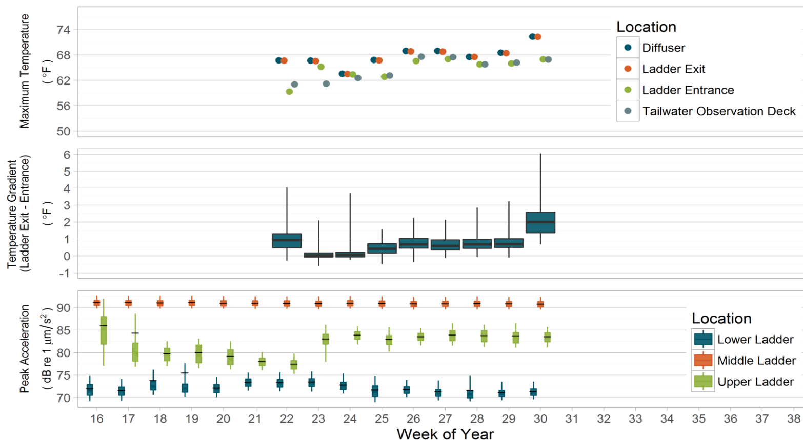
Figure 6 Running Summary of Weekly Temperature and Sound and Vibration in the Fish Ladder
