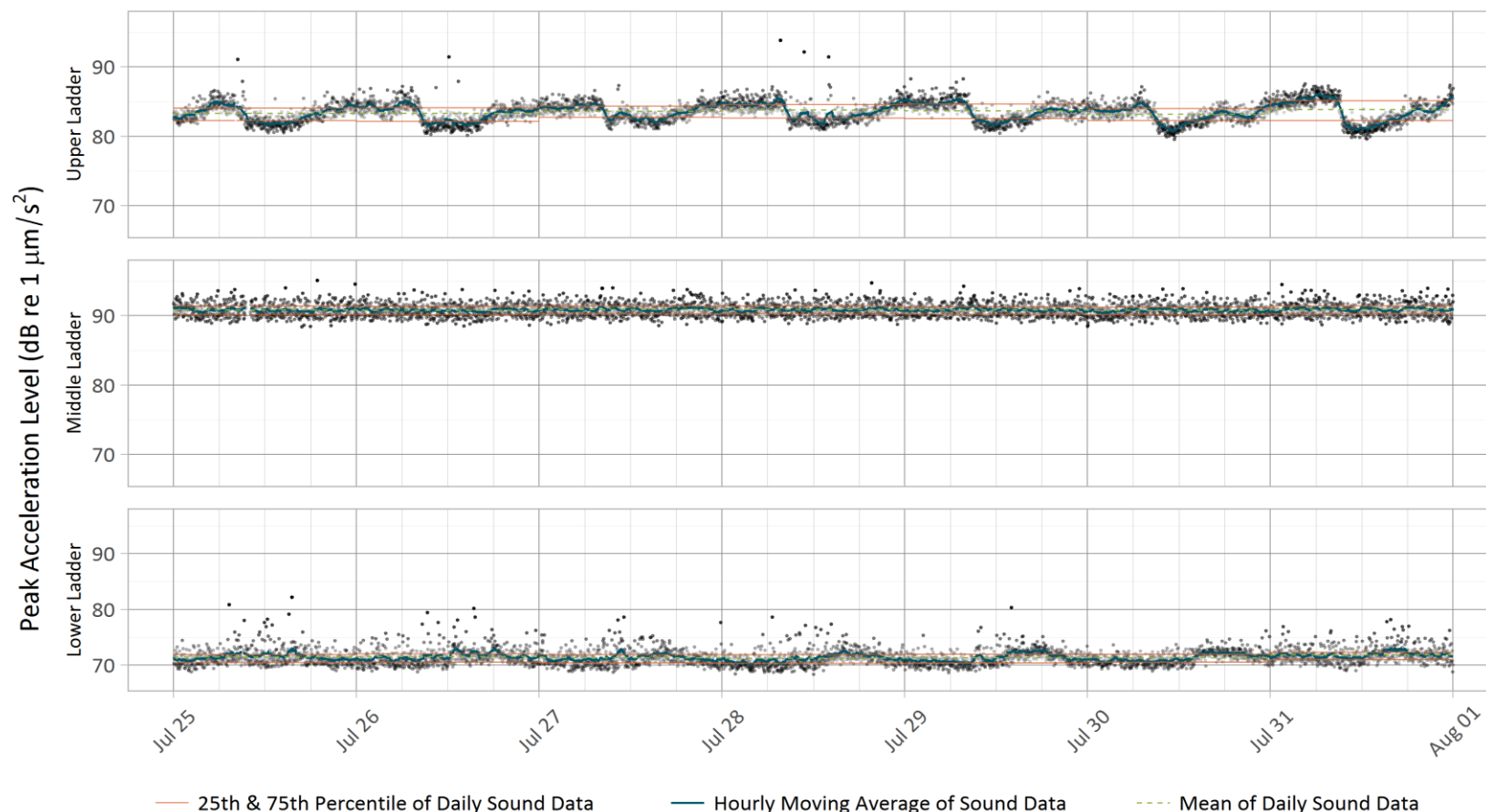
Figure 1 Peak Acceleration Levels Measured by Triaxial Accelerometers for Week 30
